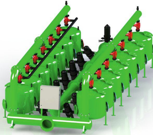
ÖZEL GRAVEL FİLTRE SİSTEM SPECIAL SAND MEDIA FILTER SYSTEM
